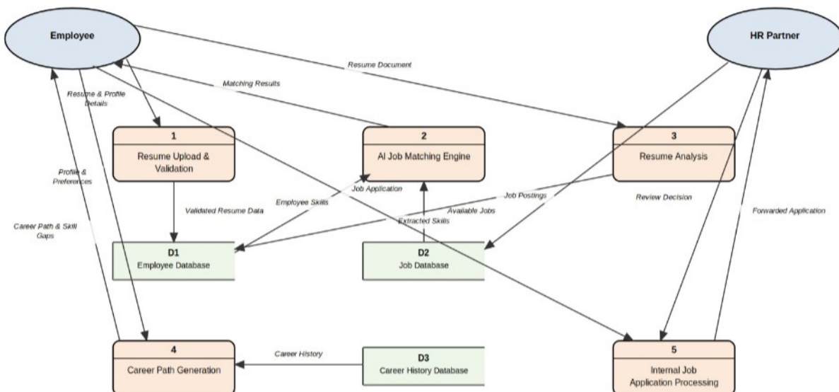
Level-1 Data Flow Diagram: Internal Job Mobility Assistant
